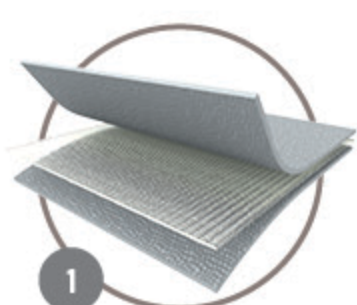
1 DURAPLUS™ CONSTRUCTION
